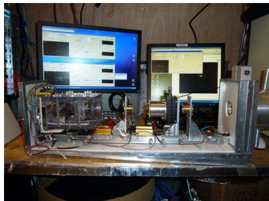
Fig. 3. Left: PBL on its telescope, observing the Sun (Oct 2011). Right: optical bench of PBL in the AstroConcordia shelter.
