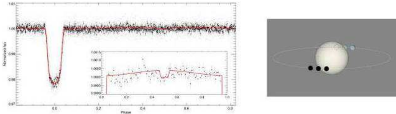
Fig. 2. (left) photometric lightcurve of WASP-19b folded at the planet period (0.79 days). (right) pictorial description (to scale!) of the primary transit and the occultation.
