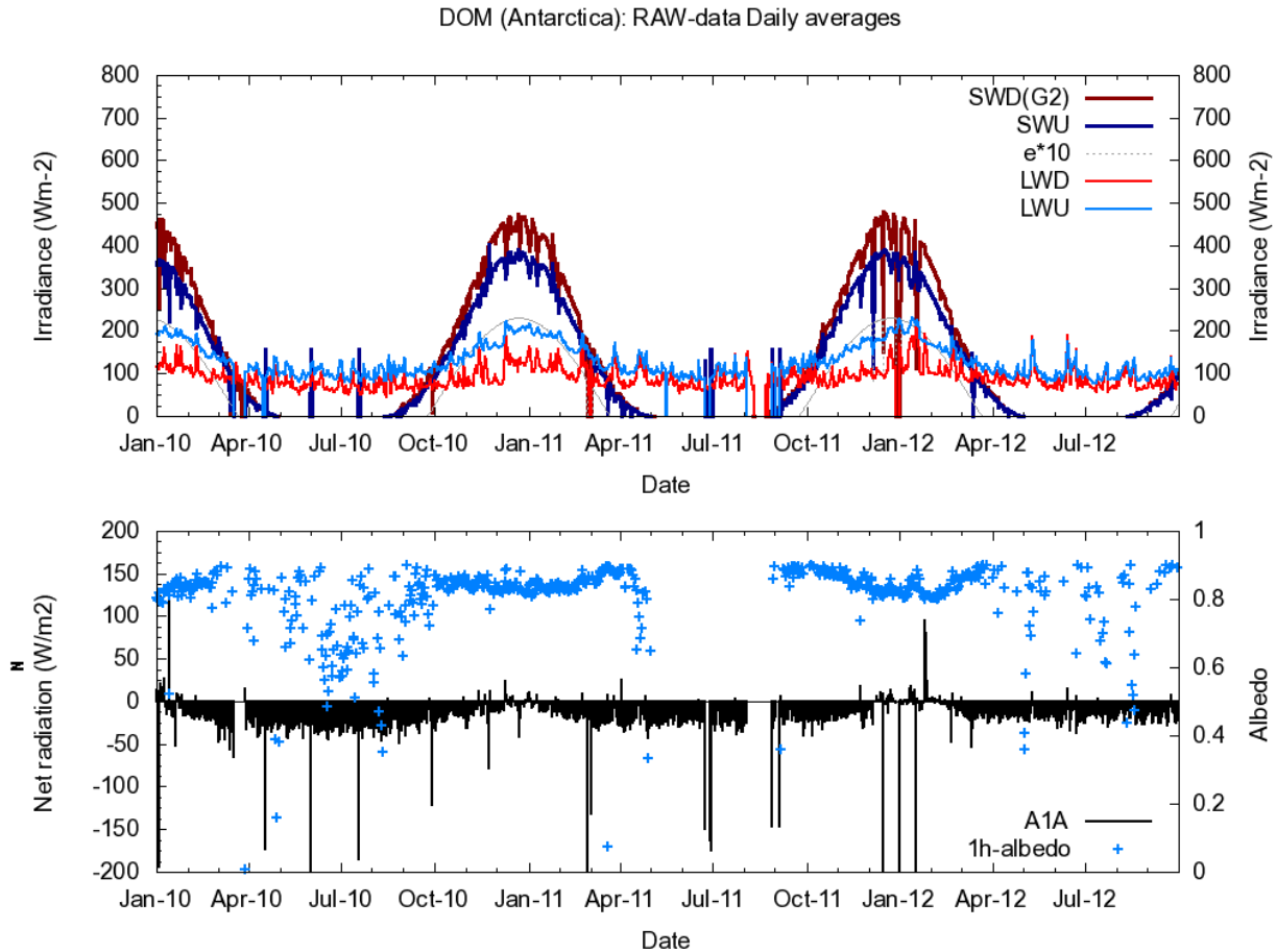
Fig. 5: Daily averages of the four components of the radiative balance at surface Upper part). Hourly averages of albedo and radiative balance at surface (lower part). Raw data. 2010-2011 and 2012 (before the last summer campaign).
