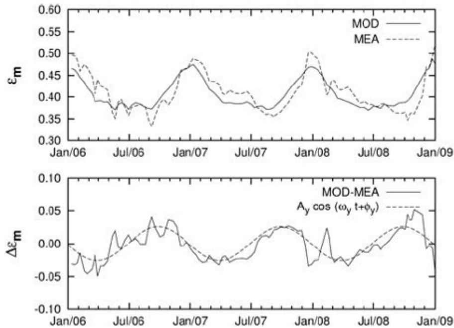
Fig. 3: Variation of the measured (MEA) and modeled (MOD) clear sky effective emissivity calculated with respect the top-inversion layer temperature T_m , at Dome C (upper part), and annual correction of the parametrization (lower part).
