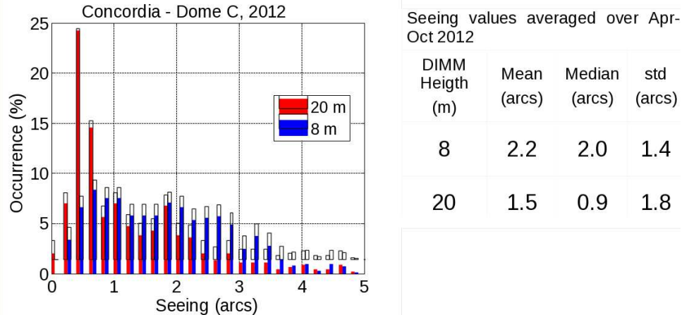
Fig. 2. Seeing statistics for DIMM (8m) and DIMM-Toit (20m) from April to October 2012.
