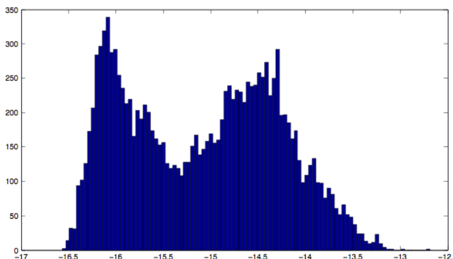
Fig. 6. Histogram of Cn2 at a height of 31m (arbitrary unit) during the month of April 2012. The bimodal structure of this histogram shows the clear separation between low turbulence (left part) and high turbulence (right part) regimes (inside or outside the planetary boundary layer). This also shows that the average height of the planetary boundary layer was approximately 31m at that period of the year (the two parts are nearly identical).
