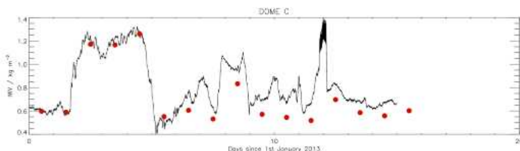
Fig. 4: Time evolution of the Integrated Water Vapour (IWV) above Dome C in 2013 as measured by the HAMSTRAD radiometer (black line), and the radiosondes (red filled circles). Note that LN 2 calibration was performed on 7 January 2013 at 08:00 UTC. The new acquisition software was installed on 8 January 2013 at 08:30 UTC.
