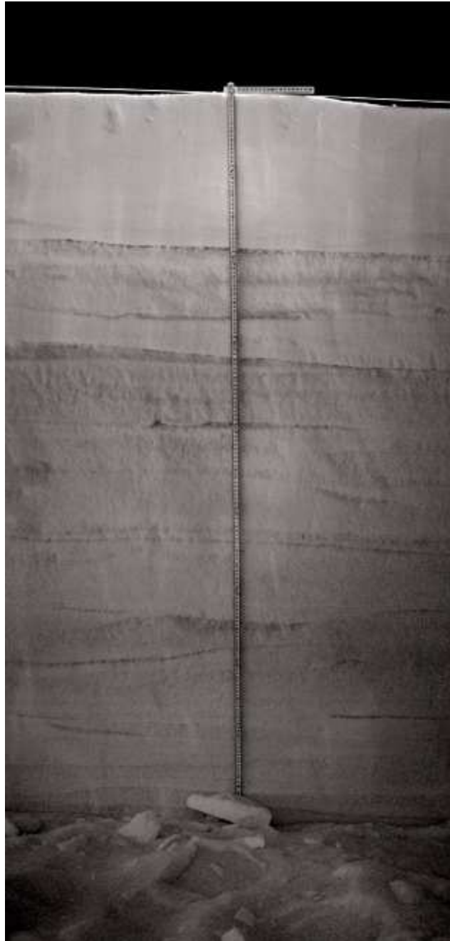
Fig. 9. Infrared image collected at the center of the trench. It can be seen that the 40 cm surface are characterized by a massive layer, consisting of very fine grains of snow. This layer is the emerged part of a "whale back".
