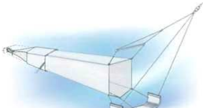
Fig. 1 – Schema di rete pelagica trainata SHPN (Small Hamburg Plankton Net)
