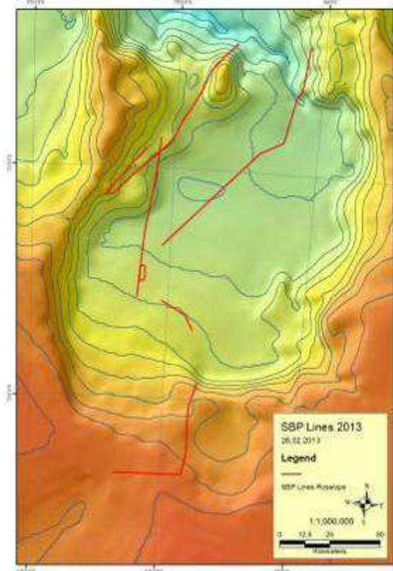
Fig 3 – Survey SBP
