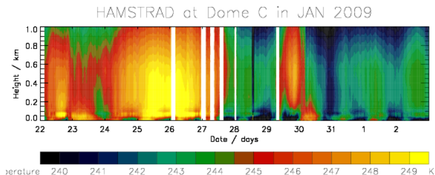
Temporal evolution of temperature from 0 to 1 km above Dome C as measured by HAMSTRAD in Boundary Layer Mode.
